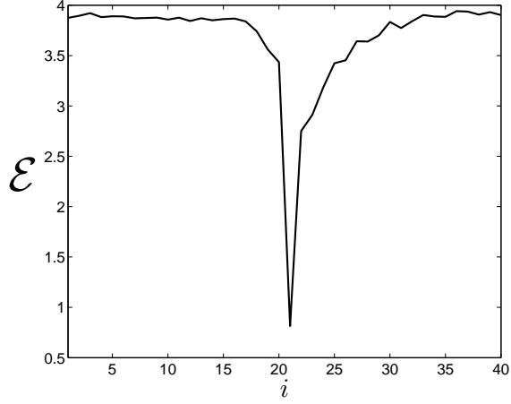
FIG. 10. RMS error \mathcal{E} for each variable z_i as a function of the lattice site i . Only one observable was used at i = 21 . Time between observations is \Delta t_{\text{obs}} = 10 hours and observational noise with covariance \mathbf{R}_o = (0.25 \sigma_{\text{clim}}^2) \mathbf{I} was used. The results are averaged over 100 different realizations.
