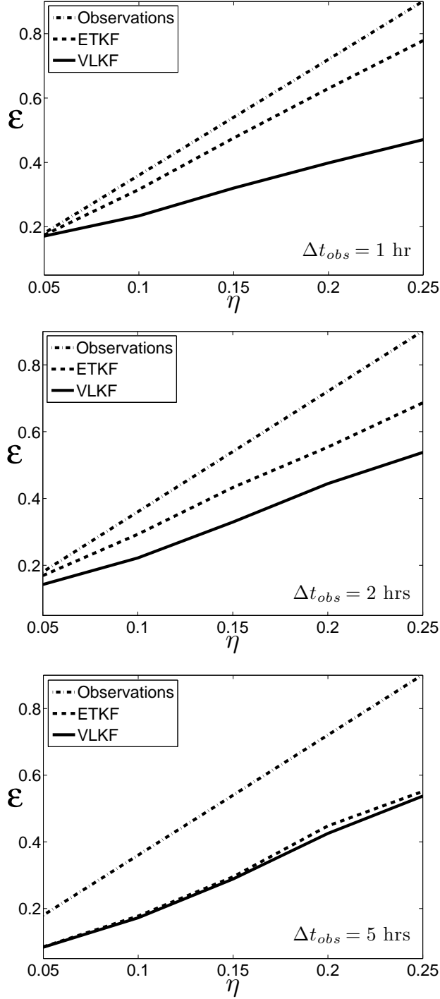
FIG. 11. Skill improvement of VLKF (solid lines), ETKF (dashed lines), as a function of the observational noise, measured here by \eta defined via \mathbf{R}_o = (\eta \sigma_{clim})^2 \mathbf{I} . The dotted line indicates the skill if only observations were used. We show results from top to bottom for several observation intervals: \Delta t_{obs} = 1 hour, \Delta t_{obs} = 2 hours and \Delta t_{obs} = 5 hours. N_{obs} = 4 was used and 1000 simulations were carried out to perform the ensemble averages in the RMS errors \mathcal{E} using (25) for ETKF and VLKF.
