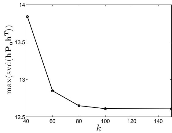
FIG. 6. Average maximal singular value of \mathbf{h}\mathbf{P}_a\mathbf{h}^T as a function of ensemble size k for the Lorenz-96 model (24), using standard ETKF without inflation and all other parameters as in Figure 4. We used 150 realisations for the averaging.
