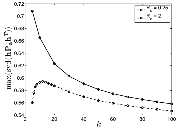
FIG. 2. Average maximal singular value of \mathbf{hP}_a \mathbf{h}^T as a function of ensemble size k for the stochastic linear toy model (12) using standard ETKF without inflation, with \mathbf{R}_o = 0.25 (dashed curve) and \mathbf{R}_o = 2 (solid curve). Parameters are \sigma_x = \sigma_y = \gamma_x = \gamma_y = 1 , \lambda = 0.2 , \Delta t_{\text{obs}} = 1 , for which the climatic variance is \mathbf{h}\Sigma \mathbf{h}^T \approx 0.505 . We used 50 realizations for the averaging.
