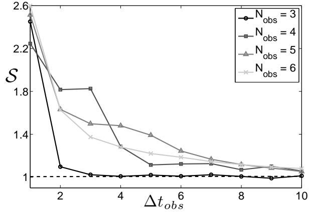
FIG. 7. Proportional skill improvement of VLKF over ETKF as a function of the observation interval \Delta t_{obs} for different values of N_{obs} , with observational noise \mathbf{R}_o = (0.25\sigma_{clim})^2 \mathbf{I} . A total of 500 simulations were used to perform the ensemble average in the RMS errors \mathcal{E} using (25) for ETKF and VLKF. \Delta t_{obs} is measured in hours.
