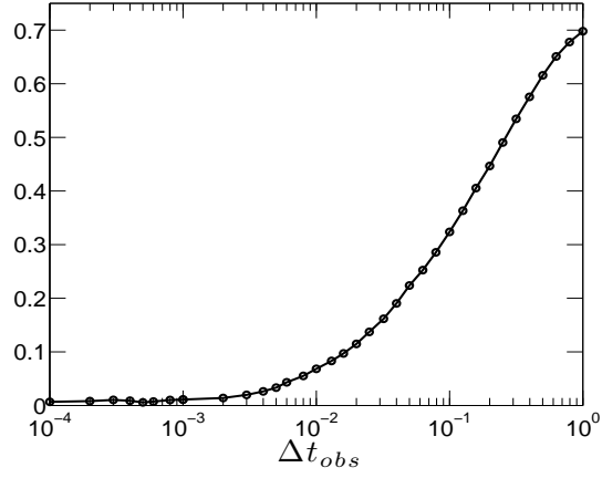
FIG. 1. Proportion of incidences when the variance constraint is switched on and \mathbf{R}_w is positive definite as a function of the observation interval \Delta t_{obs} for the stochastic linear toy model (12). We used \gamma_x = 1 , \gamma_y = 1 , \sigma_x = 1 , \sigma_y = 1 , \lambda = 0.2 . We used k = 20 ensemble members, 100 realizations and \mathbf{R}_o = \mathbf{H}\Sigma_{\text{clim}}\mathbf{H}^T and no inflation with \delta = 1 . The analytically calculated critical observation interval according to equation (16) is \Delta t_{obs} = 10^{-2} .
