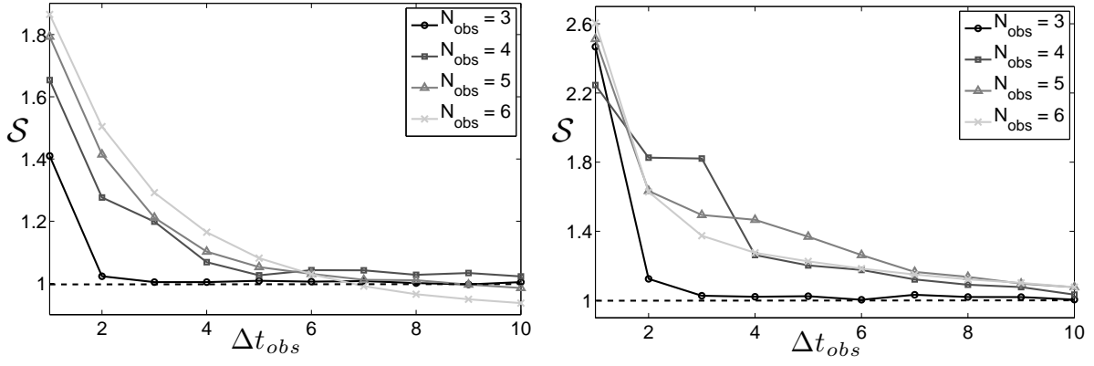
FIG. 8. Proportional skill improvement of VLKF over ETKF as a function of the observation interval \Delta t_{obs} for different values of N_{obs} . The RMS error \mathcal{E} is calculated using only the observed variables (left) or only the pseudo-observables (right). \Delta t_{obs} is measured in hours. Parameters as in Figure 7.
