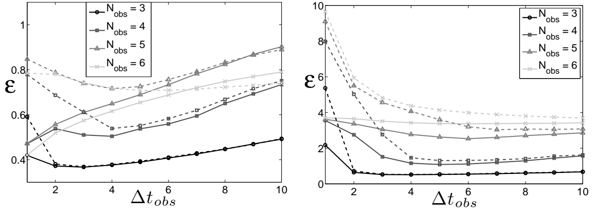
FIG. 9. RMS error of VLKF (solid lines) and ETKF (dashed lines) for \mathbf{R}_o = (0.25\sigma_{clim})^2 \mathbf{I} , where \mathcal{E} is calculated using only the observed variables (left) or only the pseudo-observables (right). \Delta t_{obs} is measured in hours. Parameters as in Figure 7.
