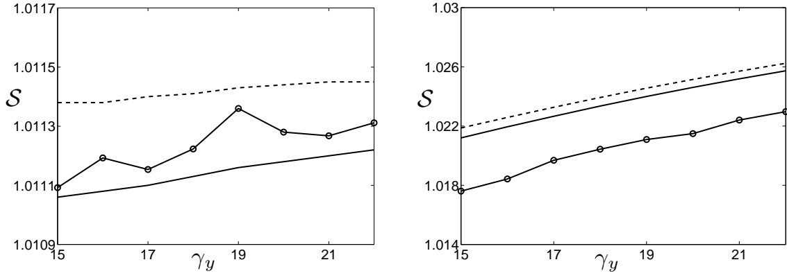
FIG. 3. Dependency of the skill improvement \mathcal{S} of VLKF over ETKF on the damping coefficient \gamma_y of the pseudo-observable. We show a comparison of direct numerical simulations (open circles) with analytical results using (21) (continuous curve) and the approximation of large ensemble size (23) (dashed curve). Parameters are \gamma_x = 1 , \lambda = 2 , \sigma_x = \sigma_y = 1 , R_{\text{obs}} = 0.25 . We used an ensemble size of k = 20 and averaged over 1000 realizations. Left: no inflation with \delta = 1 . Right: Inflation with \delta = 1.02^2 .
