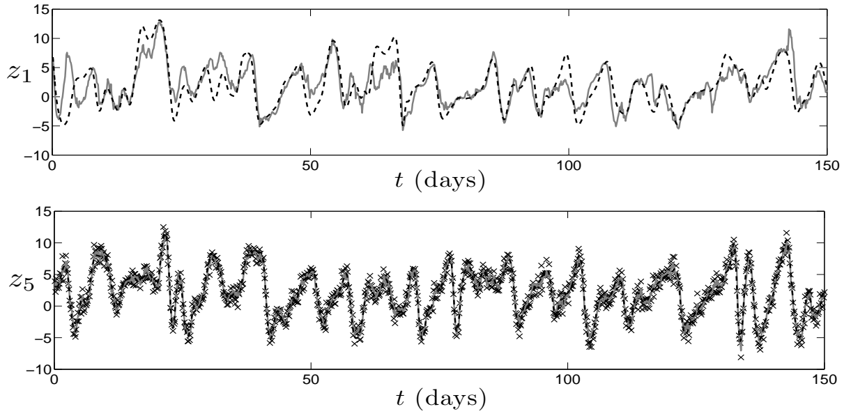
FIG. 5. Sample VLKF analysis (continuous grey line) for observed z_5 (bottom panel) and unobserved z_1 (top panel) component. The dashed line is the truth, the crosses are observations. Parameters as in Figure 4.
