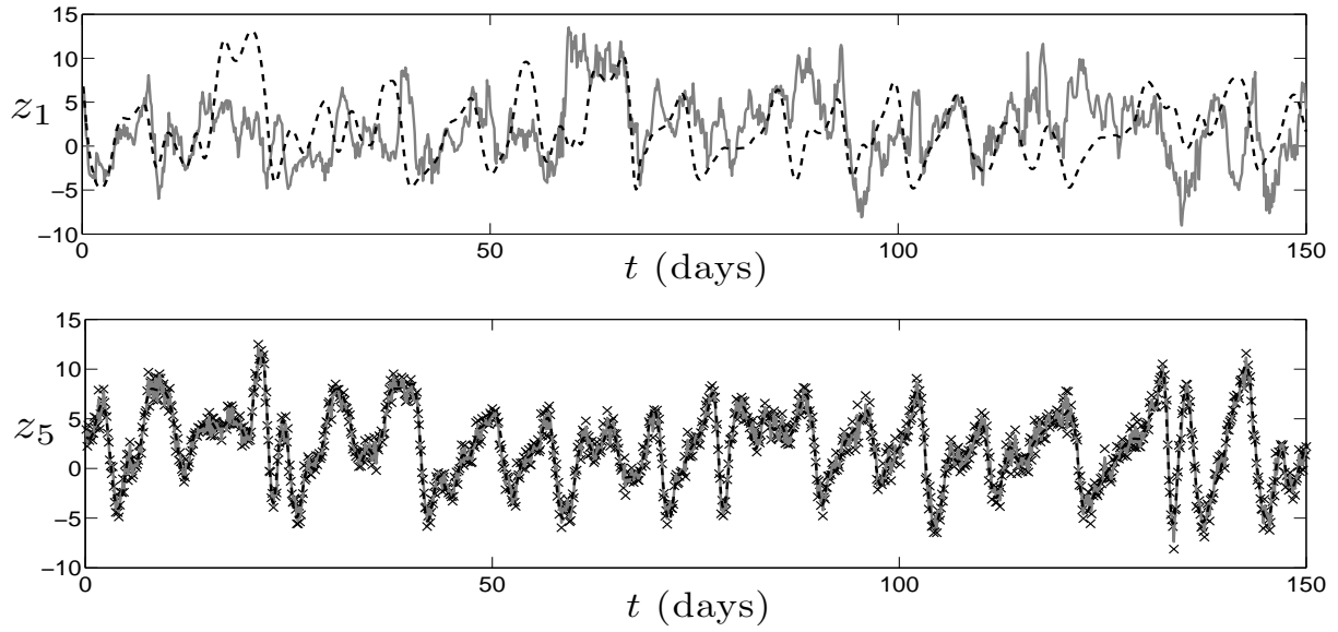
FIG. 4. Sample ETKF analysis (continuous grey line) for observed z_5 (bottom panel) and unobserved z_1 (top panel) component. The dashed line is the truth, the crosses are observations. Parameters used were N_{obs} = 5 , \Delta t_{obs} = 0.15 (18 hours) and \mathbf{R}_o = (0.25\sigma_{clim})^2 \mathbf{I} .
