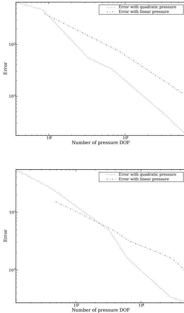
Fig. 6. Figure showing error plots for Poisson equation tests in two (upper plot) and three (lower plot) dimensions. Error is plotted against the number of pressure DOF, for the Dirichlet condition tests only. The results using the P1_D - P2 element pair are shown as dotted lines and the results using the P1_D - P1 element pair are shown as dash-dotted lines. The P1_D - P2 is more accurate (although with the same error scaling) than the P1_D - P1 element.
